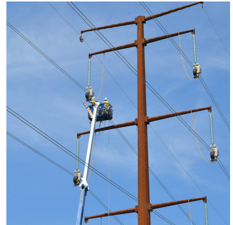
Construction will use cranes and other means to transport and install equipment (345-kV construction shown here)
